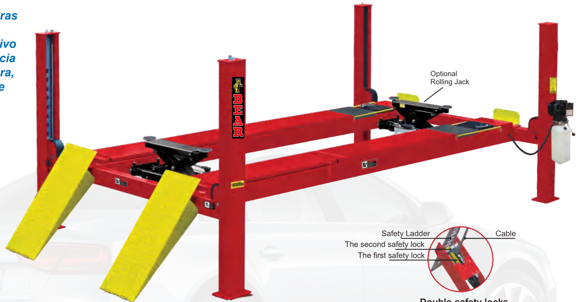
Double-safety locks
